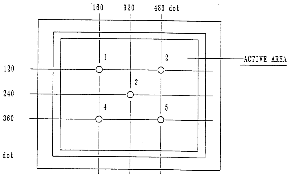
Fig. 11 Measuring points (1~5)
