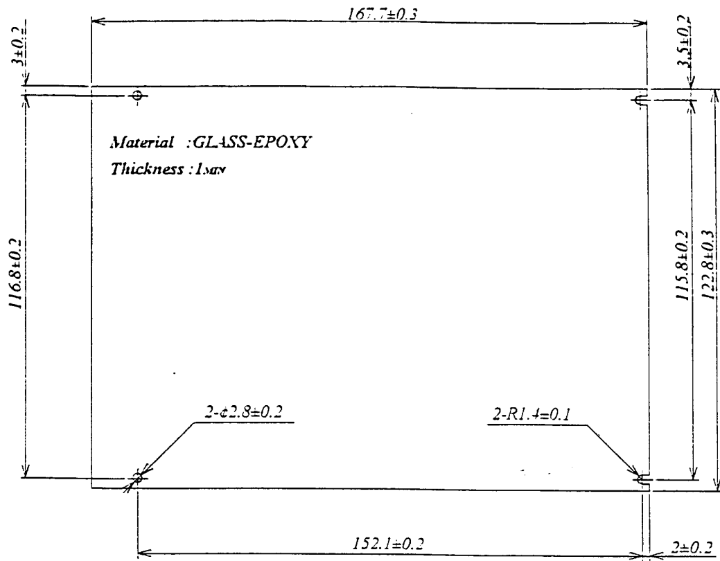
Fig13 Outline Dimensions of Recommended digitizer board
