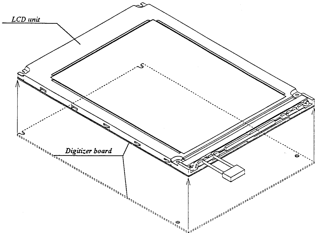
Fig14 Assembly of digitizer board
