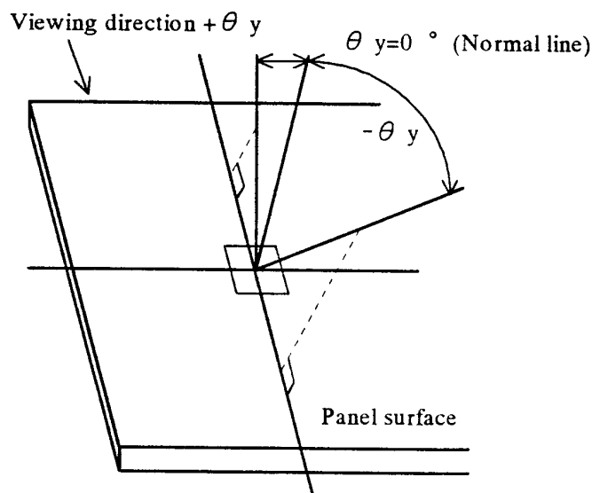
Fig.12 Definition of viewing angle
